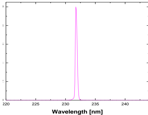
Typical 230nm Spectra
