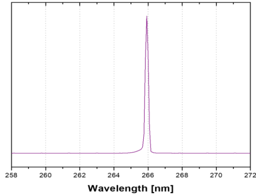
Typical 260nm Spectra
