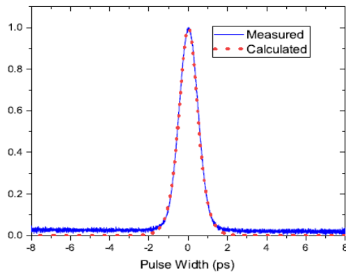
Pulse Width
